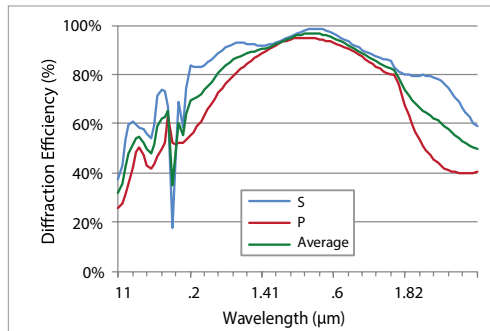
Typical absolute diffraction efficiency at AOI 49.9° *
